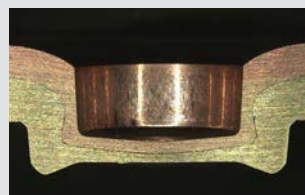
Copper in brass
